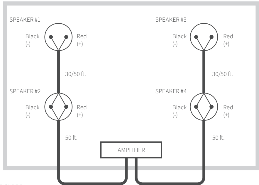
FIGURE 5: WIRING DIAGRAM
