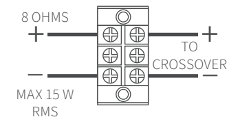
FIGURE 11: TERMINAL BLOCK
