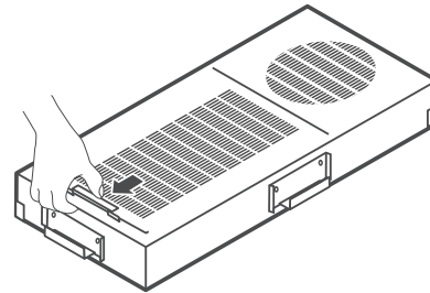
FIGURE 9A: OPEN FRONT PANEL
