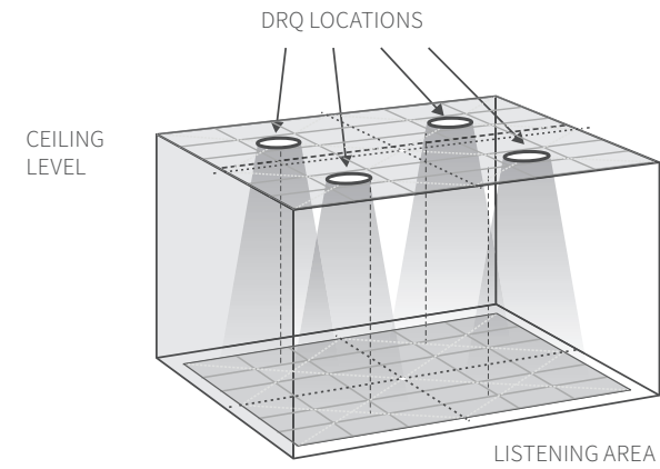
FIGURE 1: SPEAKER PLACEMENT
