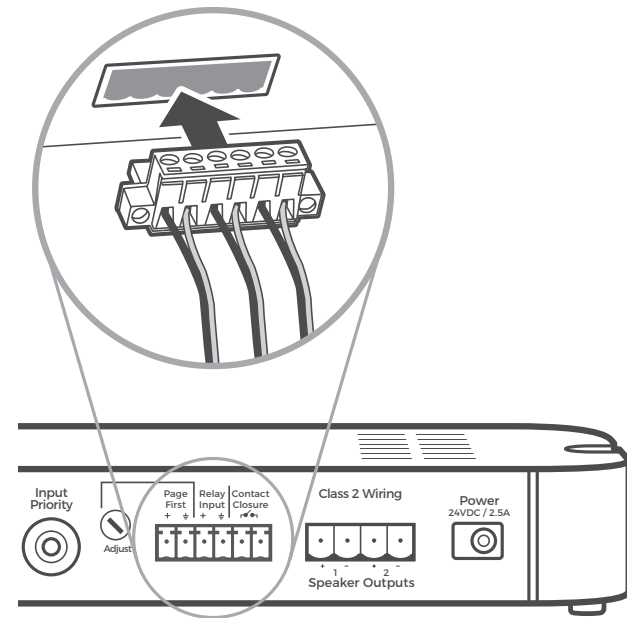
CONNECTING PAGEFIRST TO AMPLIFIER
