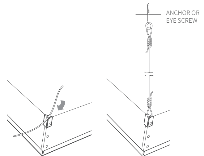
FIGURE 7: SECURE THE WIRE IN THE TWO SAFETY WIRE TABS
