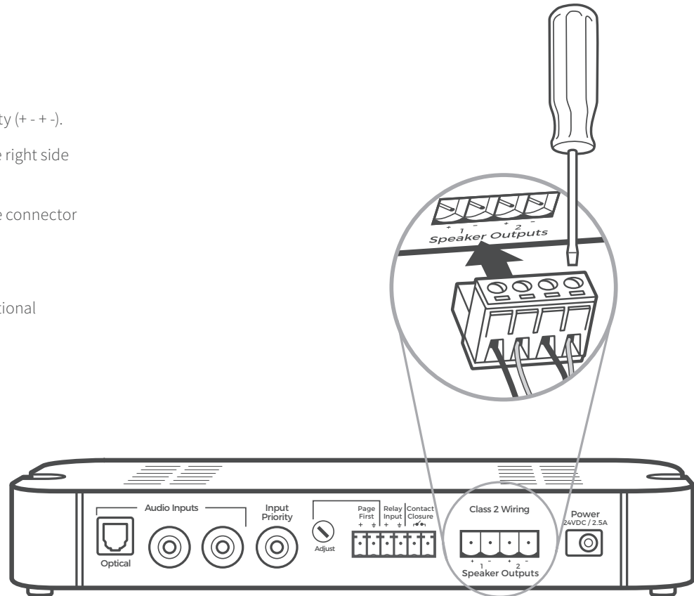
CONNECTING SPEAKER WIRES TO BACK OF THE 975
